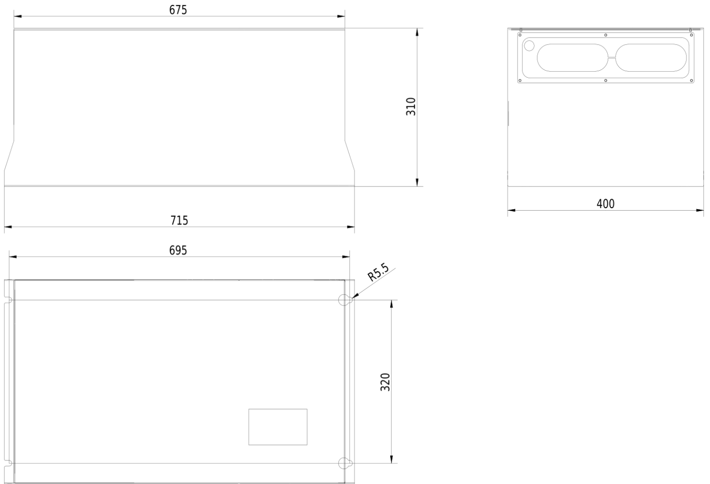
Dimensional drawing V900 - 185kW 4T1850
