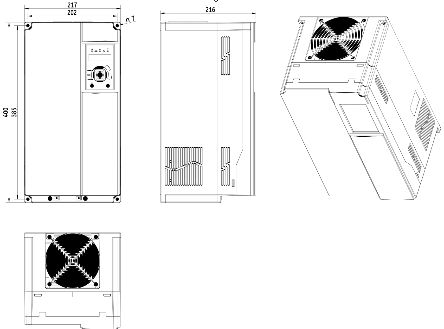
Dimensional drawing V900 - 37kW 4T0370
