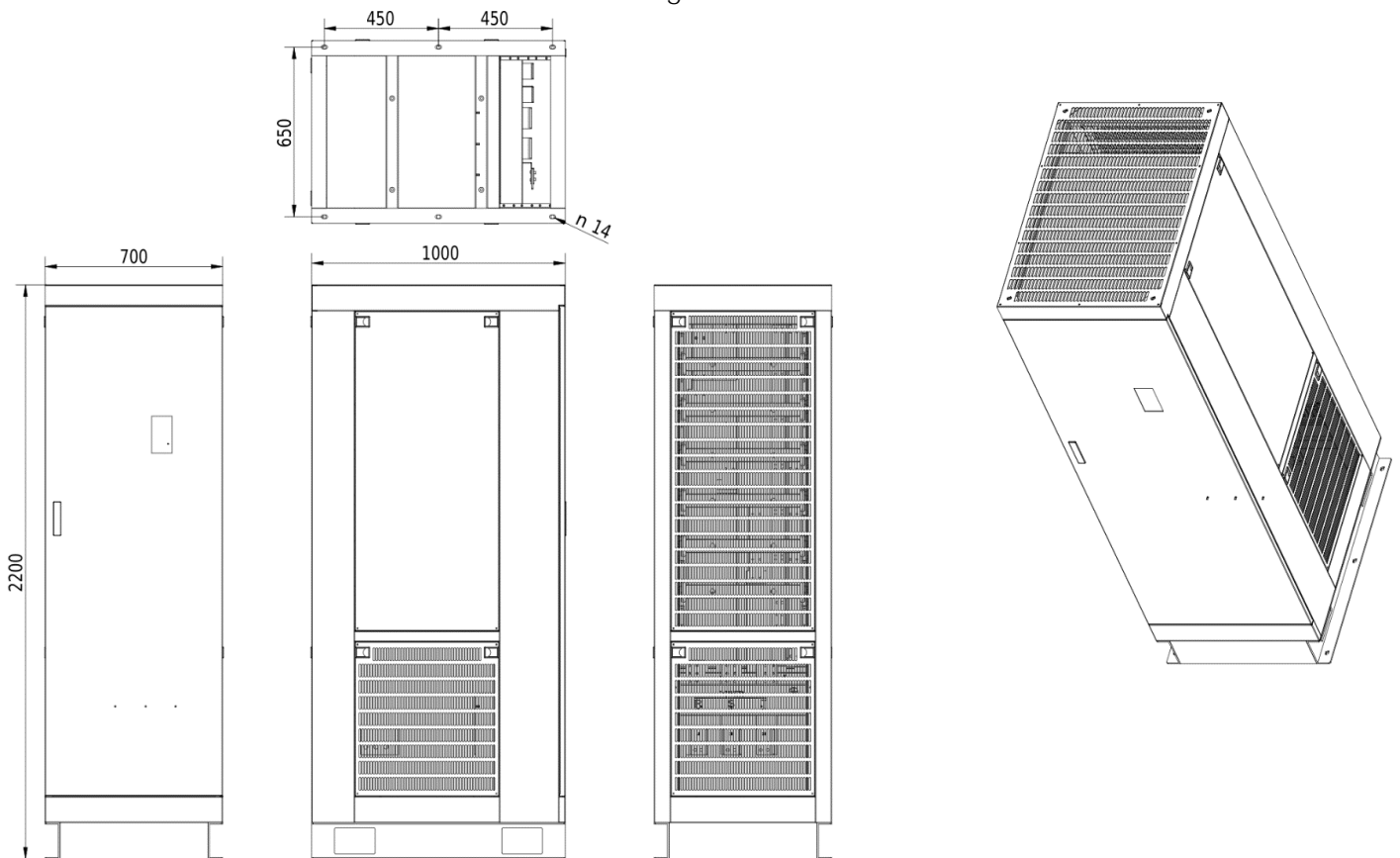
Dimensional drawing V810 - 900kW 4T9000
