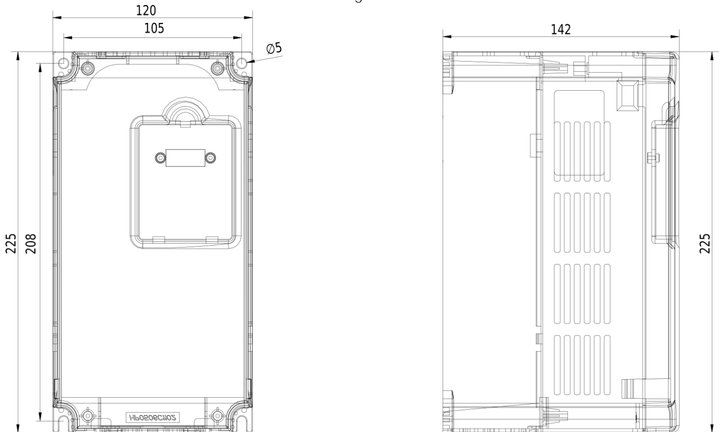
Dimensional drawing V810 - 3kW 4T0030
